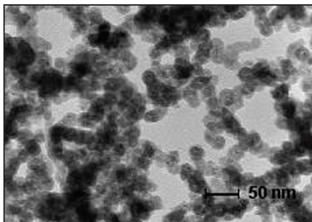
QSI-Nano® manganese is available in sizes ranging from 20 to 50 nanometers. Manganese content is controlled by oxide thickness and can range from 30% wt. to 90% wt.
